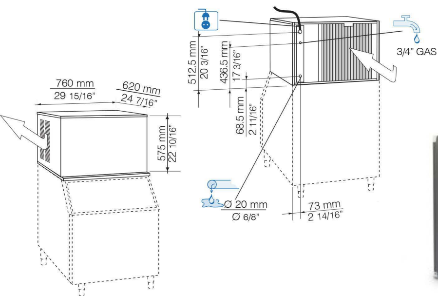
Air cooled unit
